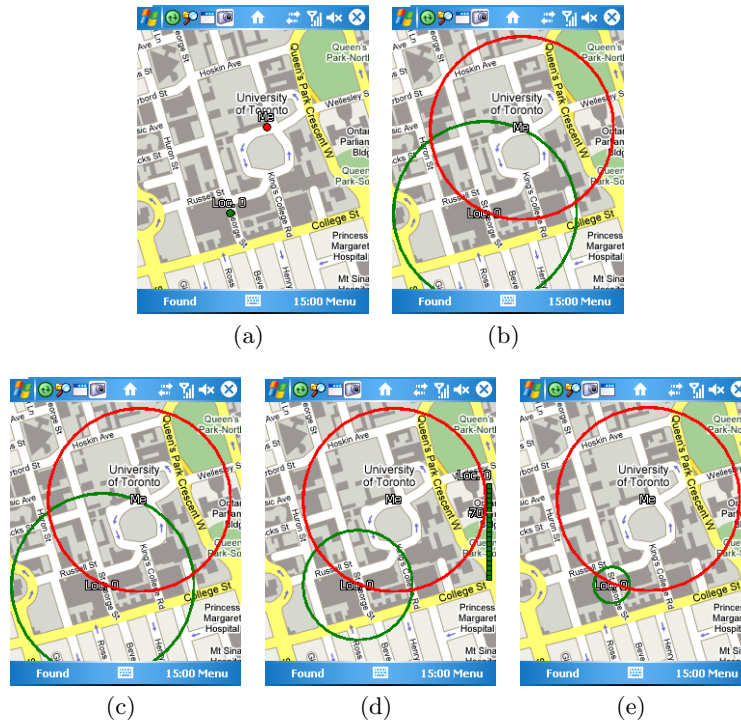
Fig. 3. The experimental four conditions: predicted location (a); 95% confidence (b); customizable confidence by default (c) and after the confidence value has been manipulated (d); and optimal error (e).
